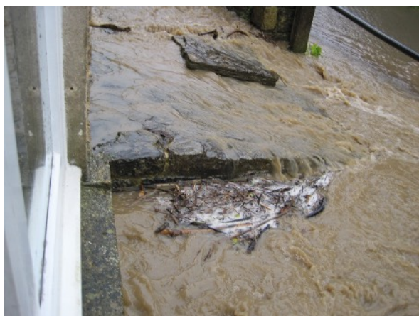
Flooding along the Brook in 2014
