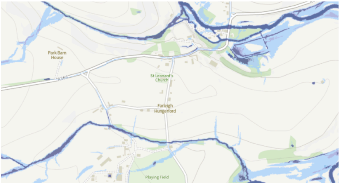
Figure 15: Surface water Flood risk in Farleigh Hungerford
